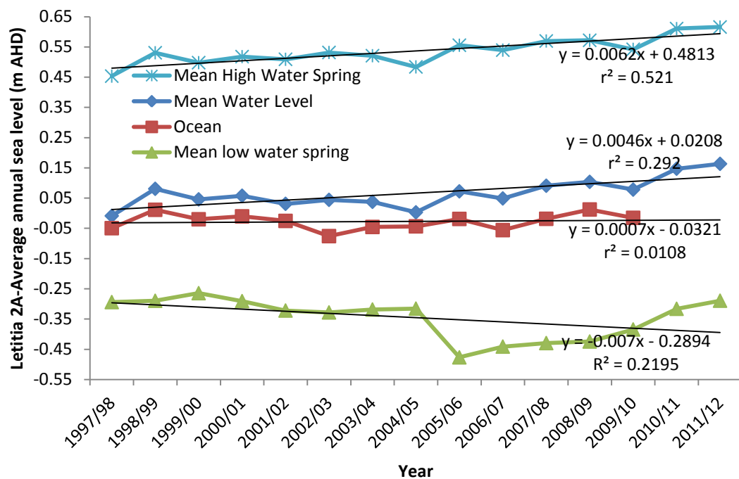
Figure 53: Annualised mean high water spring tide and mean water level at the Letitia 2A gauge within the Tweed River estuary and mean ocean water level from 1997 to 2012.
