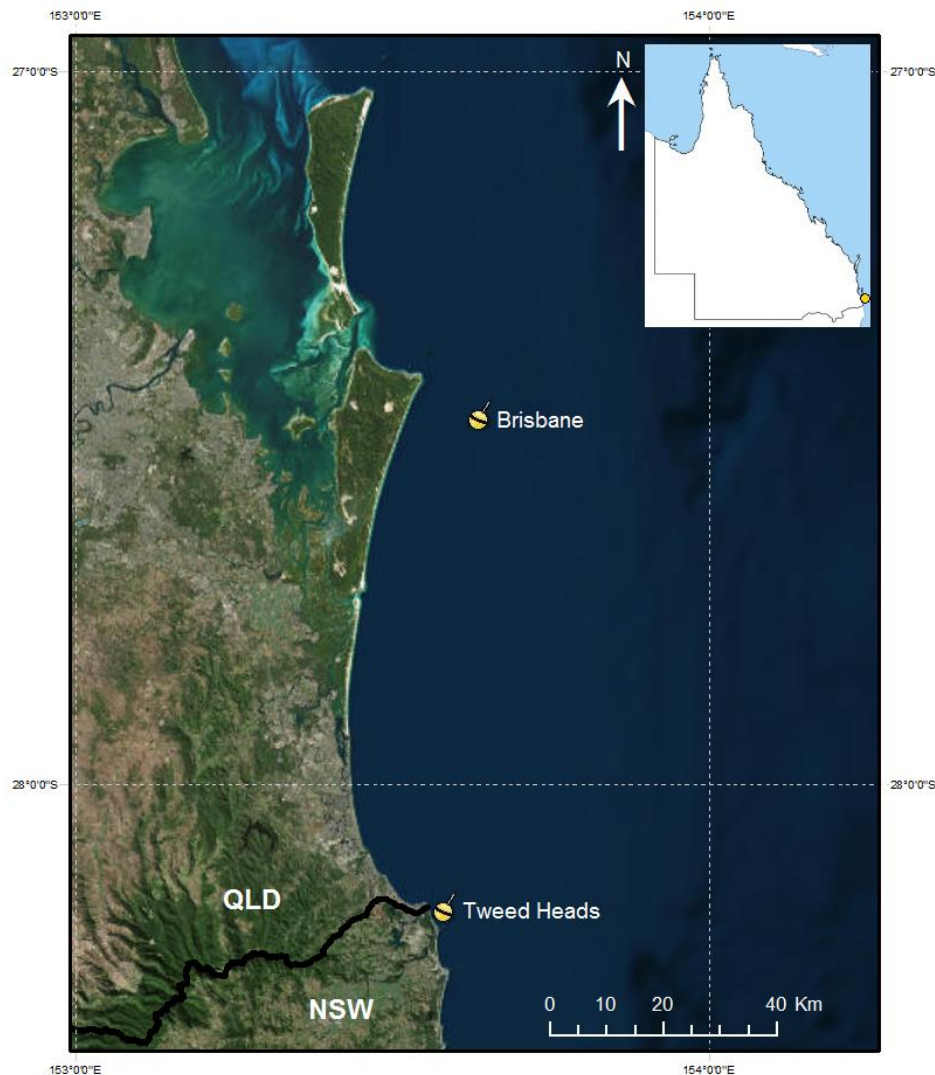
Figure 1.1: Tweed regional wave recording sites – Locality plan
