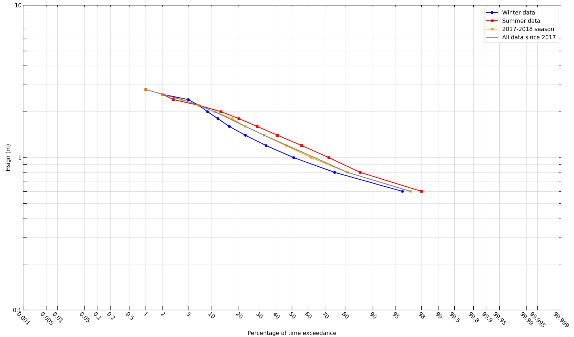
Figure 4.1: Tweed Heads MK4 Waverider buoy – Percentage (of time) exceedance of wave heights ( H_{sig} ) for all wave periods ( T_p )
