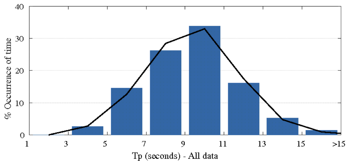
Figure 3.5: Tweed Heads Waverider buoy – Histogram percentage (of time) occurrence of wave periods (Tp) for all wave heights (Hsig)
