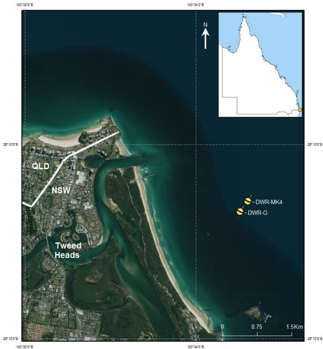
Figure 3.1: Tweed Heads DWR-G and MK4 buoys – Locality plan
